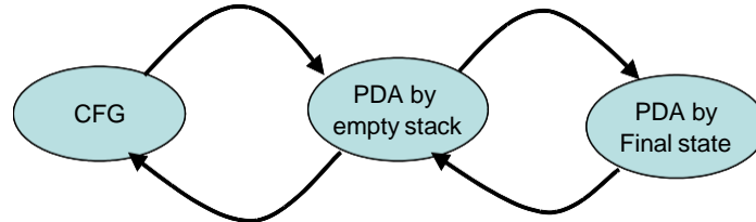
Figure 1: Equivalence of PDA and CFG
