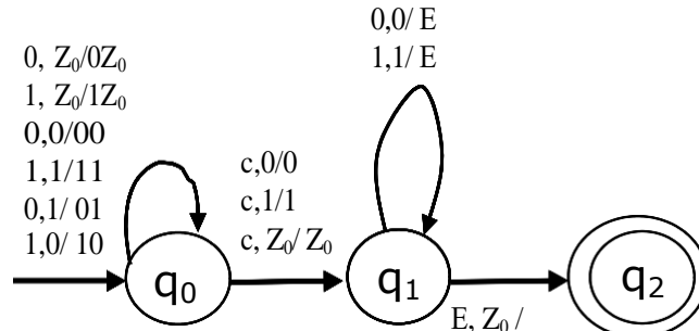
Figure 2: DPDA L = \{wcw^R\}
