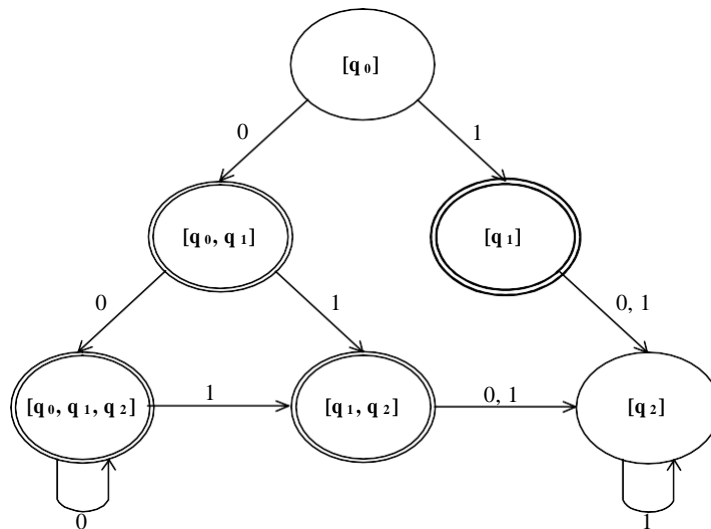
Fig.2.35 The DFA
