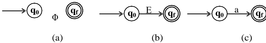
Fig 3.1 NFAs to accept \Phi , E and a
